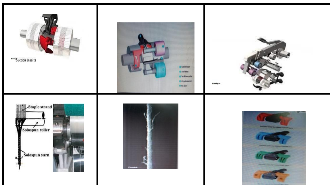
Fig. 10. K45 compact spinning frame
