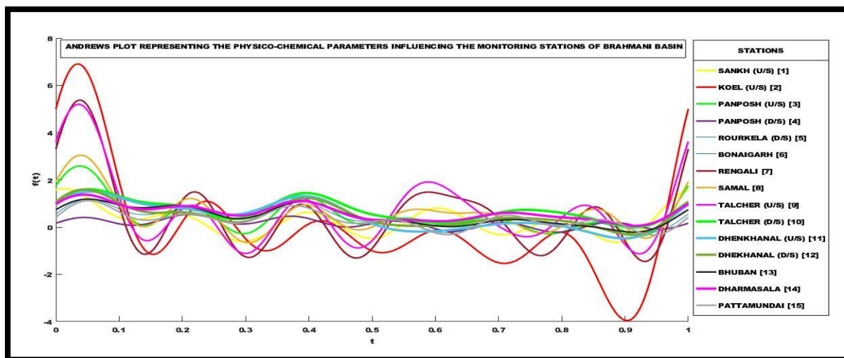
(Figure6. Andrew plots showing physico-chemical parameters and their composition of monitoring sites of the Brahmani river basin)
