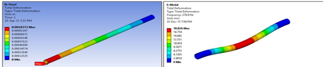
Fig.5-Total Deformation
