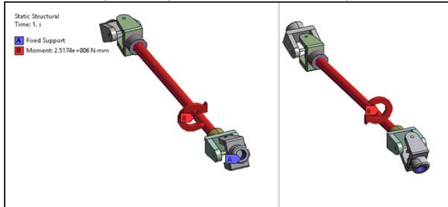
Fig.2-Boundary Conditions for the torsional analysis
