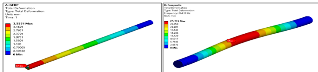
Fig.9-Total Deformation
