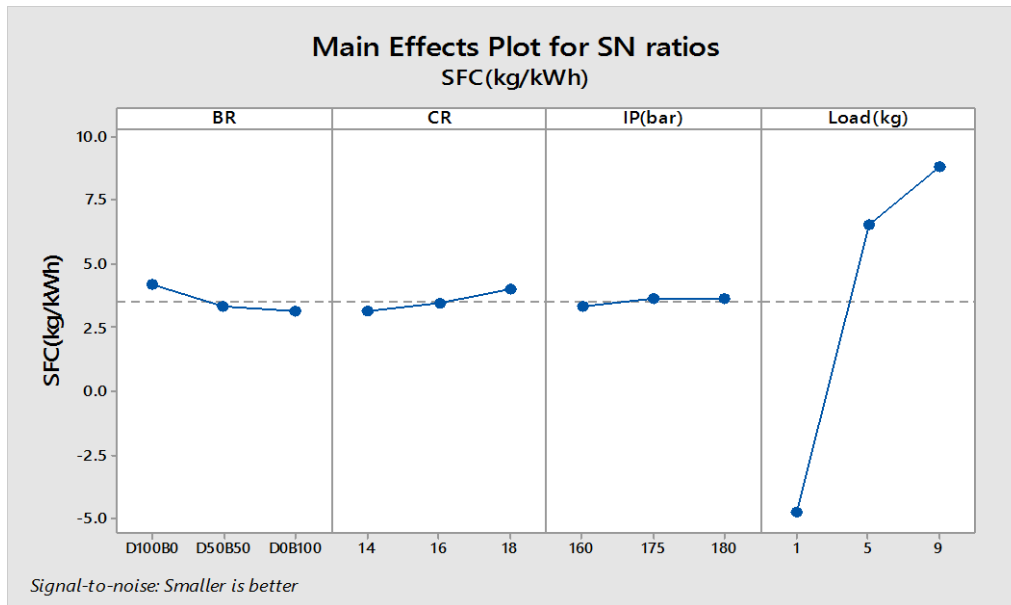
Fig 3: Main Effects Plot for SN ration for SFC
