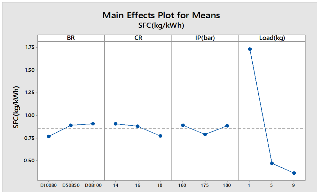
Fig 4: Main Effects Plot for Means for SFC
