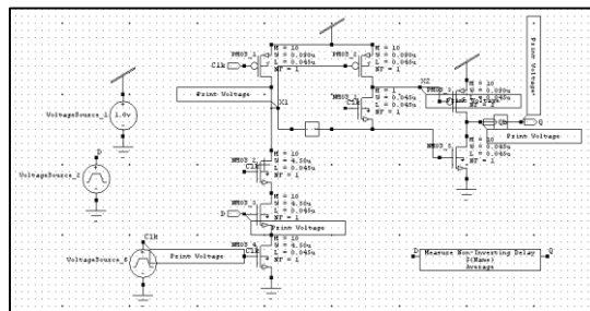
Fig 4: Schematic diagram of DDF
