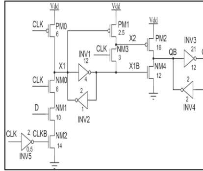
Fig 3: Circuit diagram of DDF
