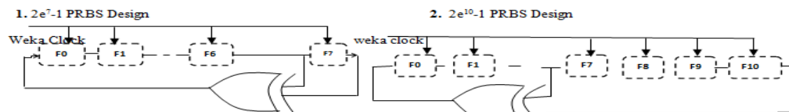
Fig. 7: 2^7-1 PRBS Design
