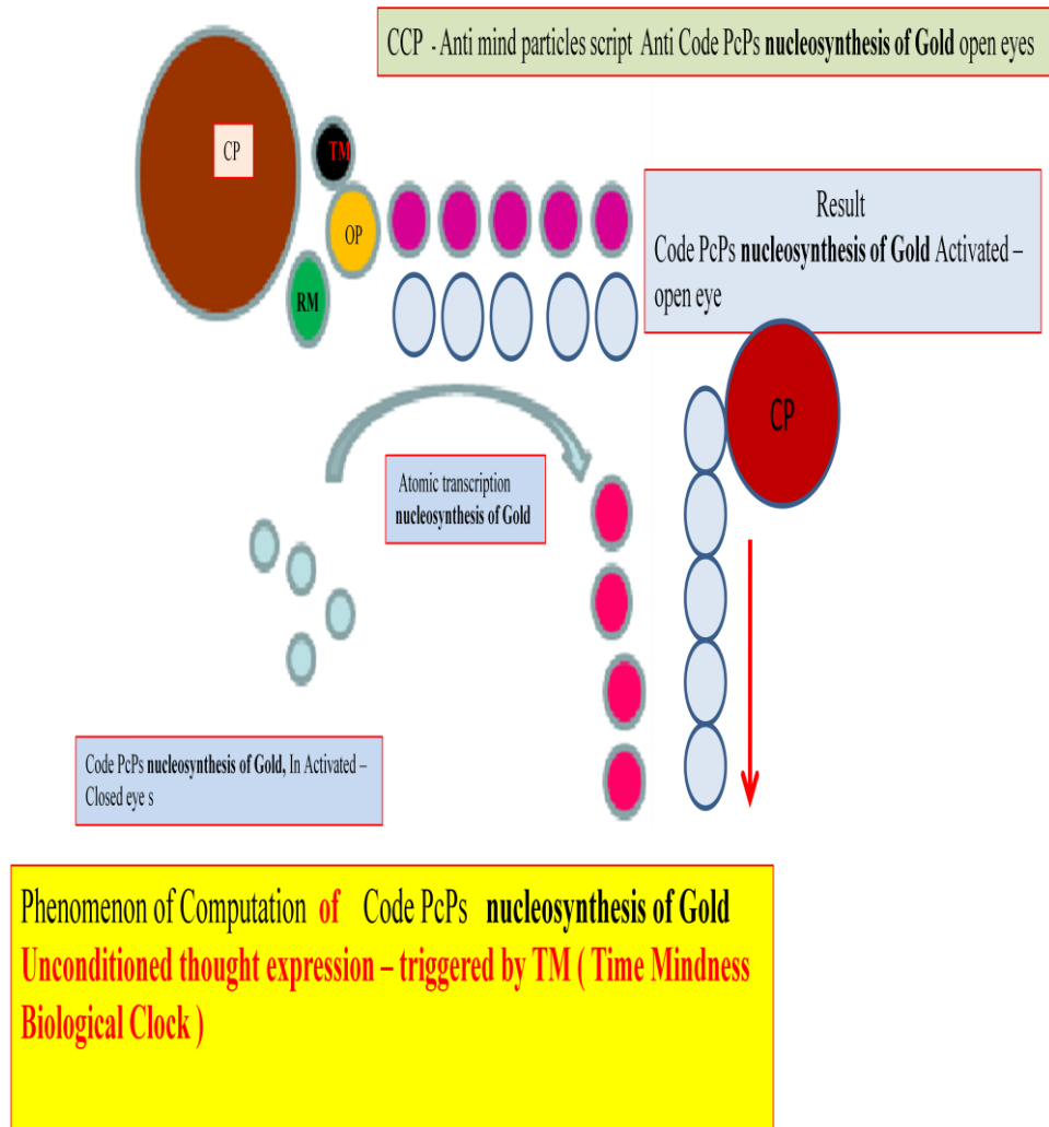
Fig 22 Phenomenon of computation of thought expression of phenomenon of nucleosynthesis of Gold ( micro level )
