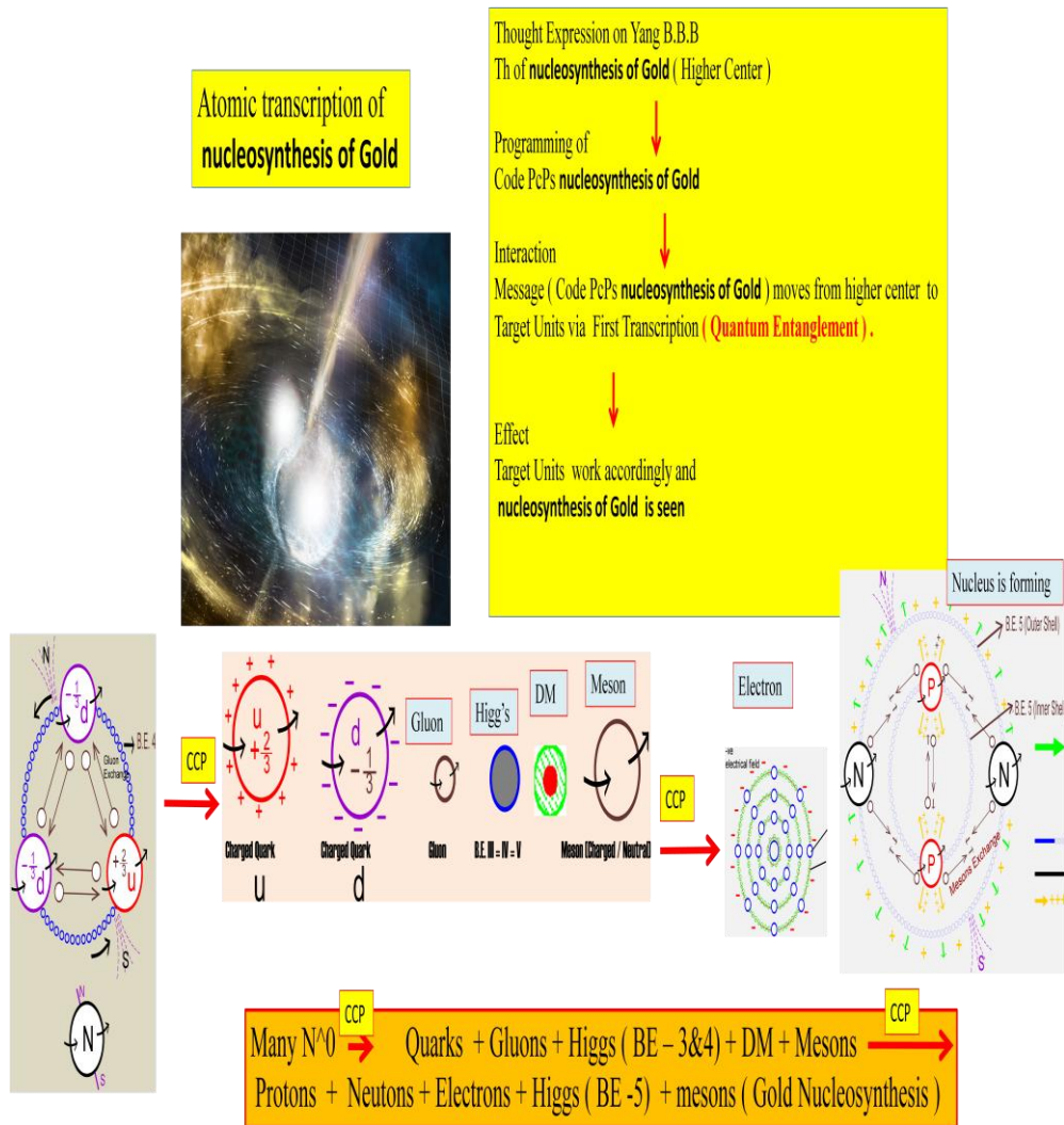
Fig 23 Nucleosynthesis of Gold , ( or uranium and platinum) atoms by unconditioned thought expression during neutron stars collision .
