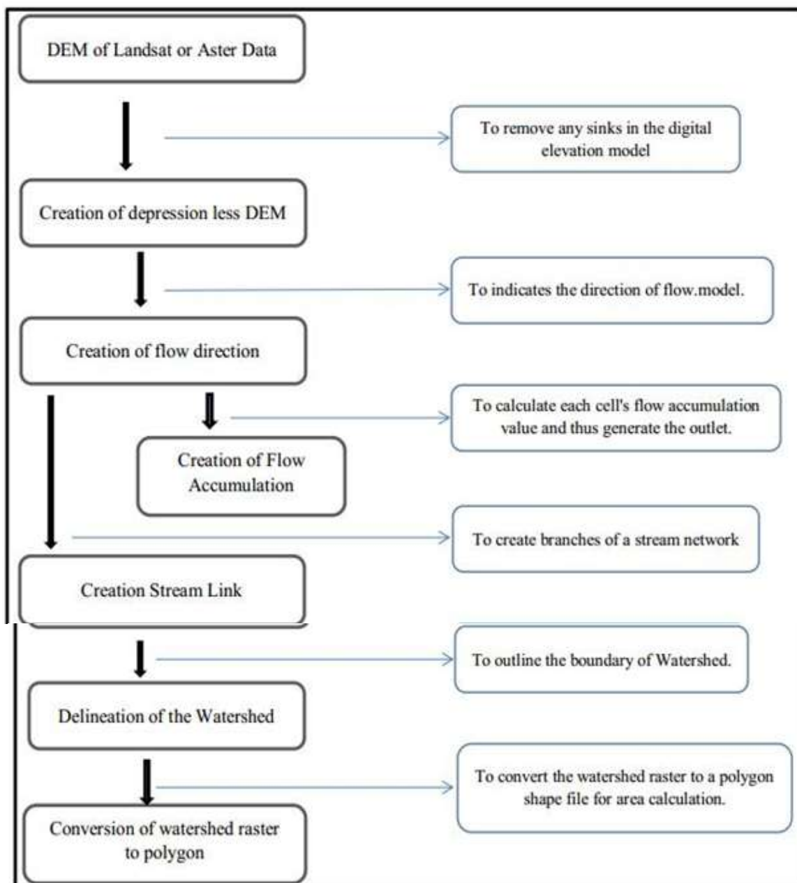
Figure 2. Outline of automatic Watershed Delineation method by ArcGIS 9.3
