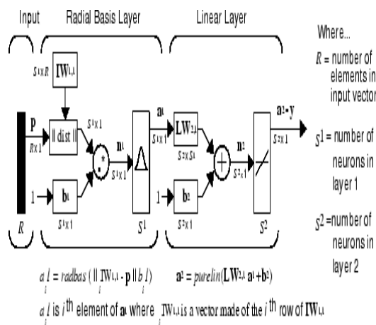
Fig. 5 Network architecture
