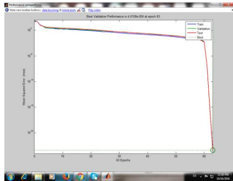
Fig. 11 Training results
