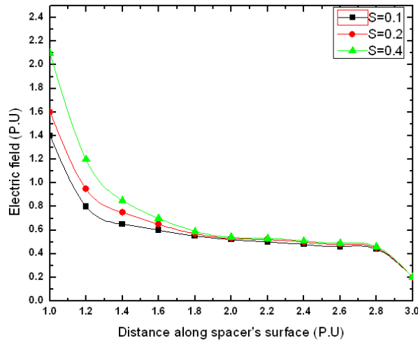
Fig. (7) Effect of spacer’s thickness on the electric field distribution along its lower surface
