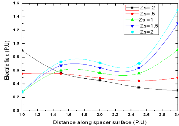
Fig. (2) Effect of Zs on the electric field distribution along the spacer surface
