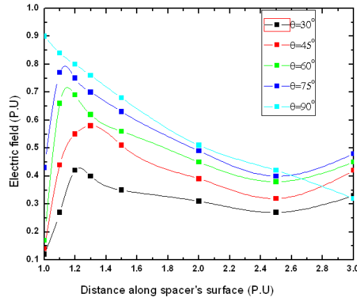
Fig. (4) Effect of inclination angle on the electric field distribution along upper cone surface
