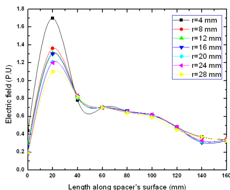
Fig. (10) Electric field distribution along concave spacer surface at different values of ( r )
