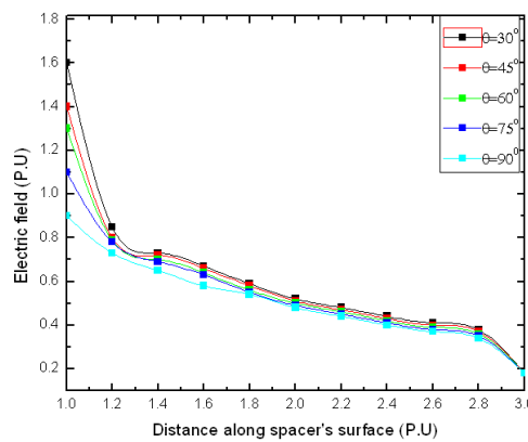
Fig.(5)Effect of inclination angle on the electric field distribution along the lower cone surface
