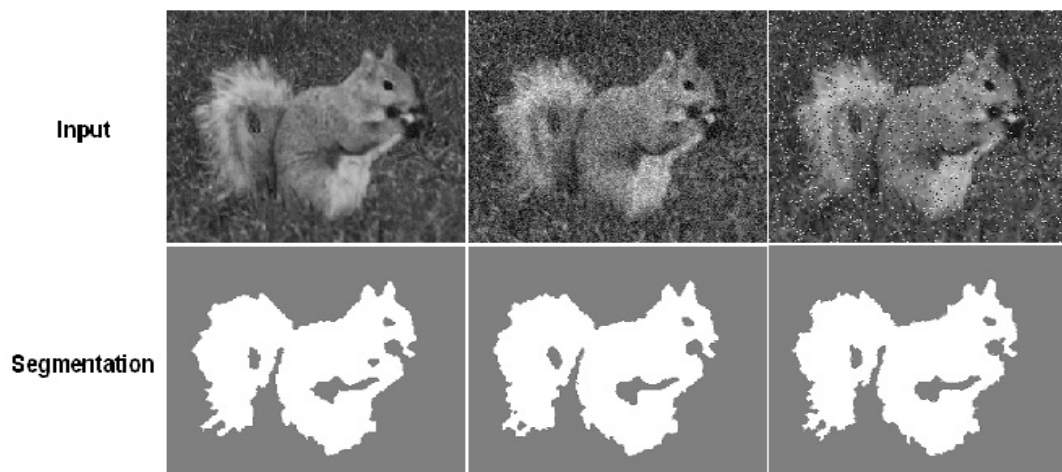
Fig. 2 Segmentation
