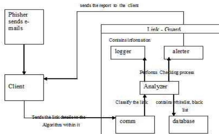
Fig 3: LINK GUARD ALGORITHM
