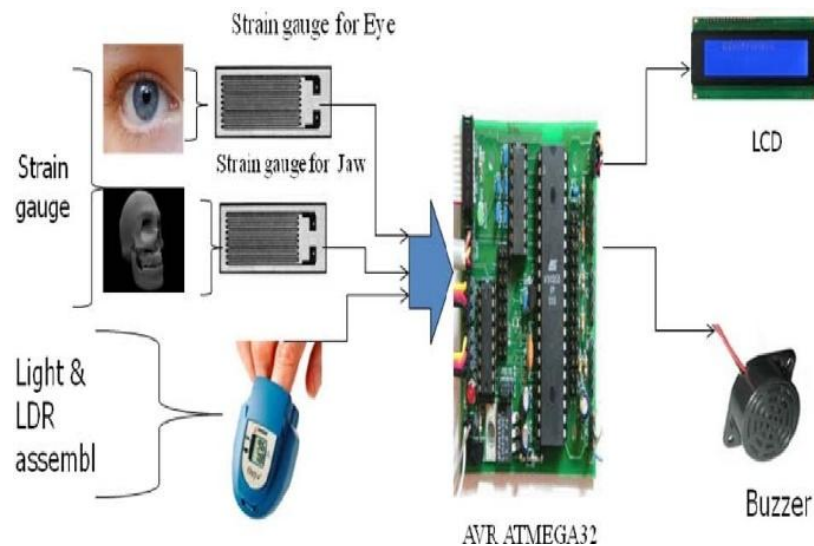
Fig1. Proposed Fatigue detection system
