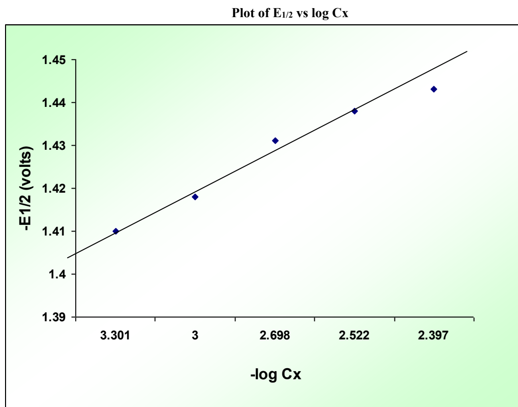
Fig. 1.3 Co(II)-Atropine Complex
