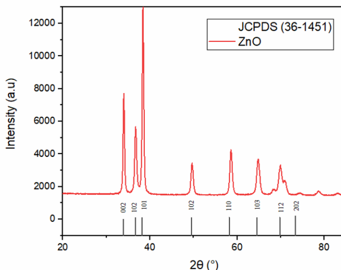
Figure 3: ZnO XRD Pattern
