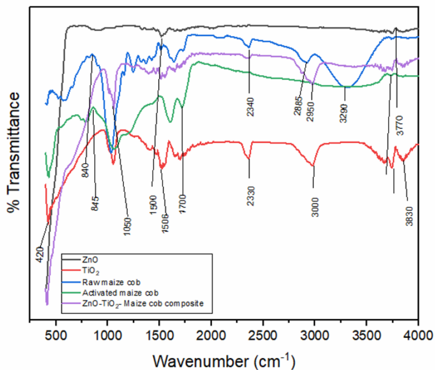
Figure 1: FTIR Spectra of \text{TiO}_2 , ZnO, and Maize Cob Nanocomposite
