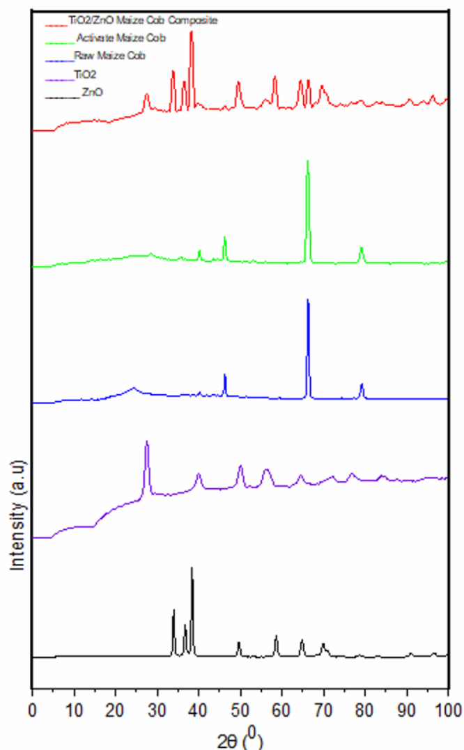
Figure 4: \text{TiO}_2/\text{ZnO} -Maize Cob Composite XRD Pattern
